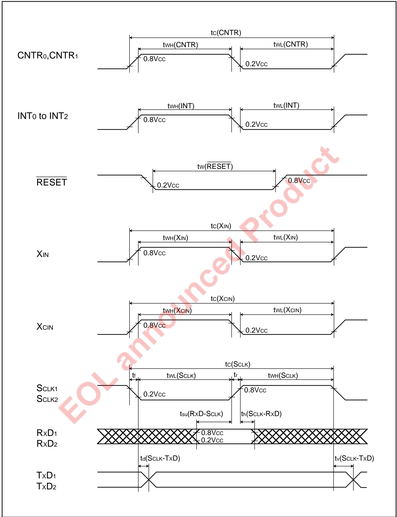
Fig. 72 Timing chart
