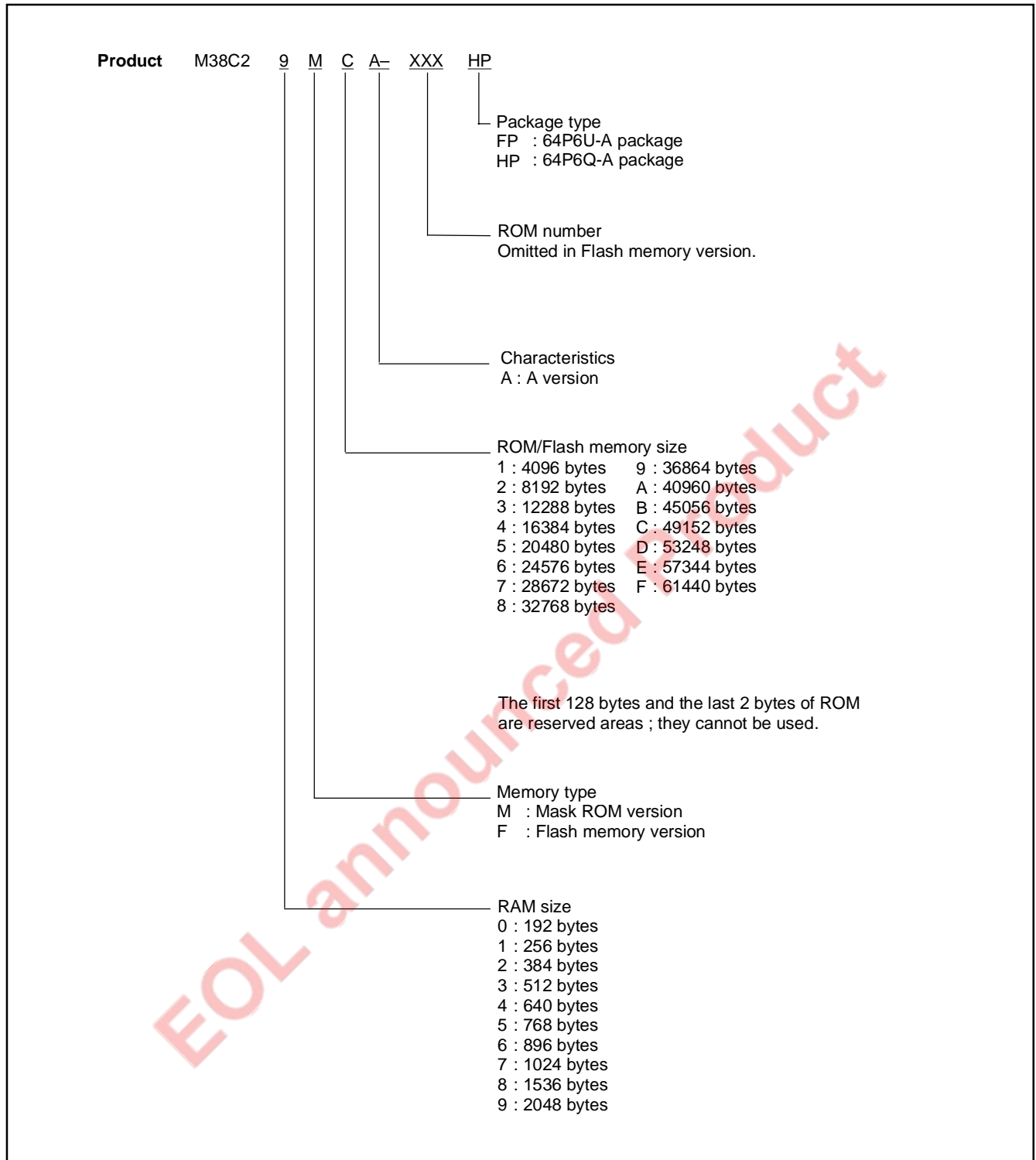
Fig. 3 Part numbering
